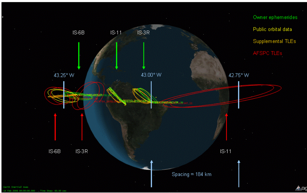
Fig. 4. Comparison of Orbital Products for Intelsat 3R, 6B, and 11
