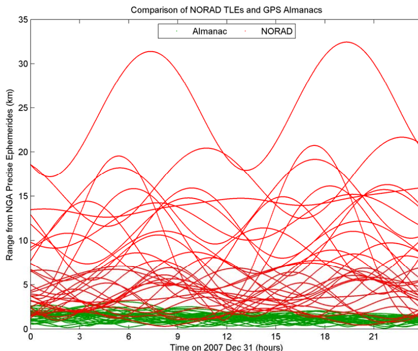
Fig. 1. Comparison of NORAD TLEs and GPS Almanacs
