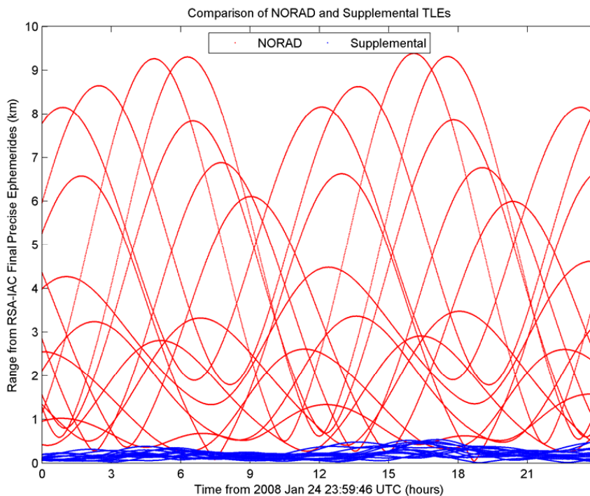
Fig. 3. Comparison of NORAD and Supplemental TLEs for GLONASS
