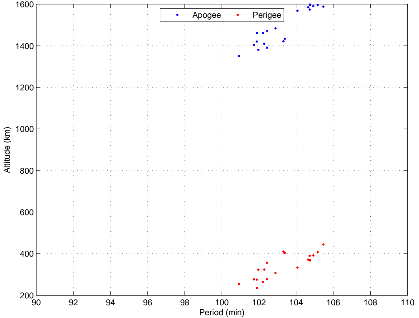
Gabbard Plot of Launch 2013-055 (20 pieces)
